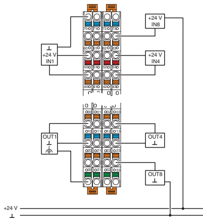
Connection diagram
