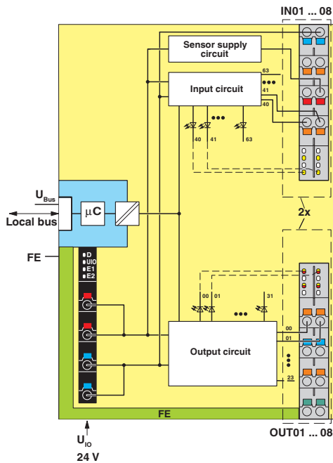
Block diagram
